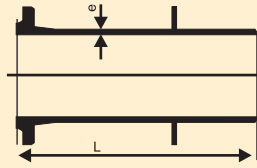
Flanged Spigot Puddle Pipe
